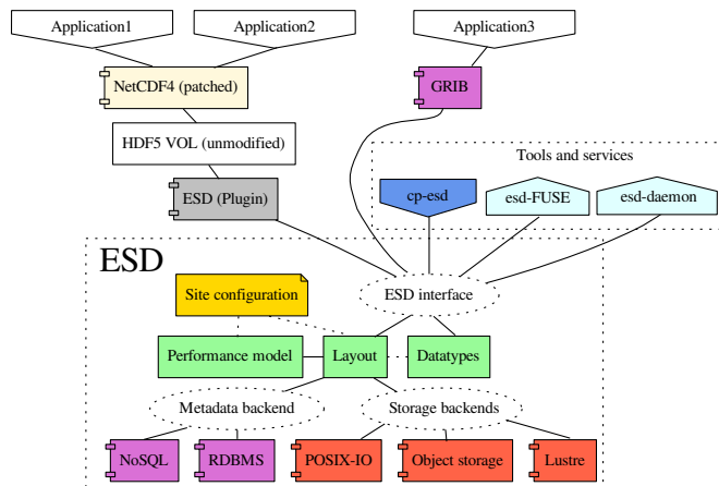
Fig. 1. Architecture overview
